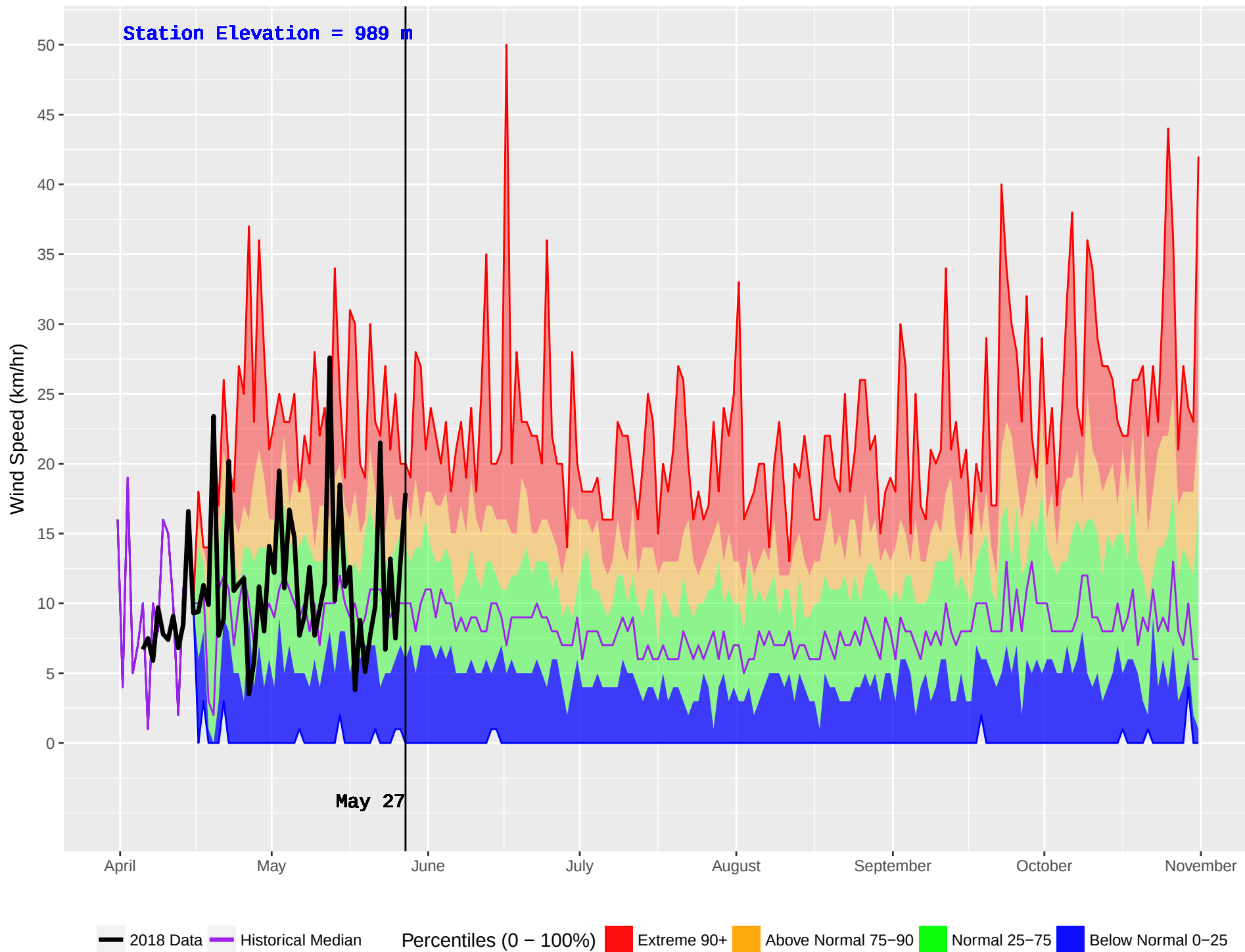
PINK MOUNTAIN (129) : Historical (1983–2016) and Current (2018) Noon Wind Speed
