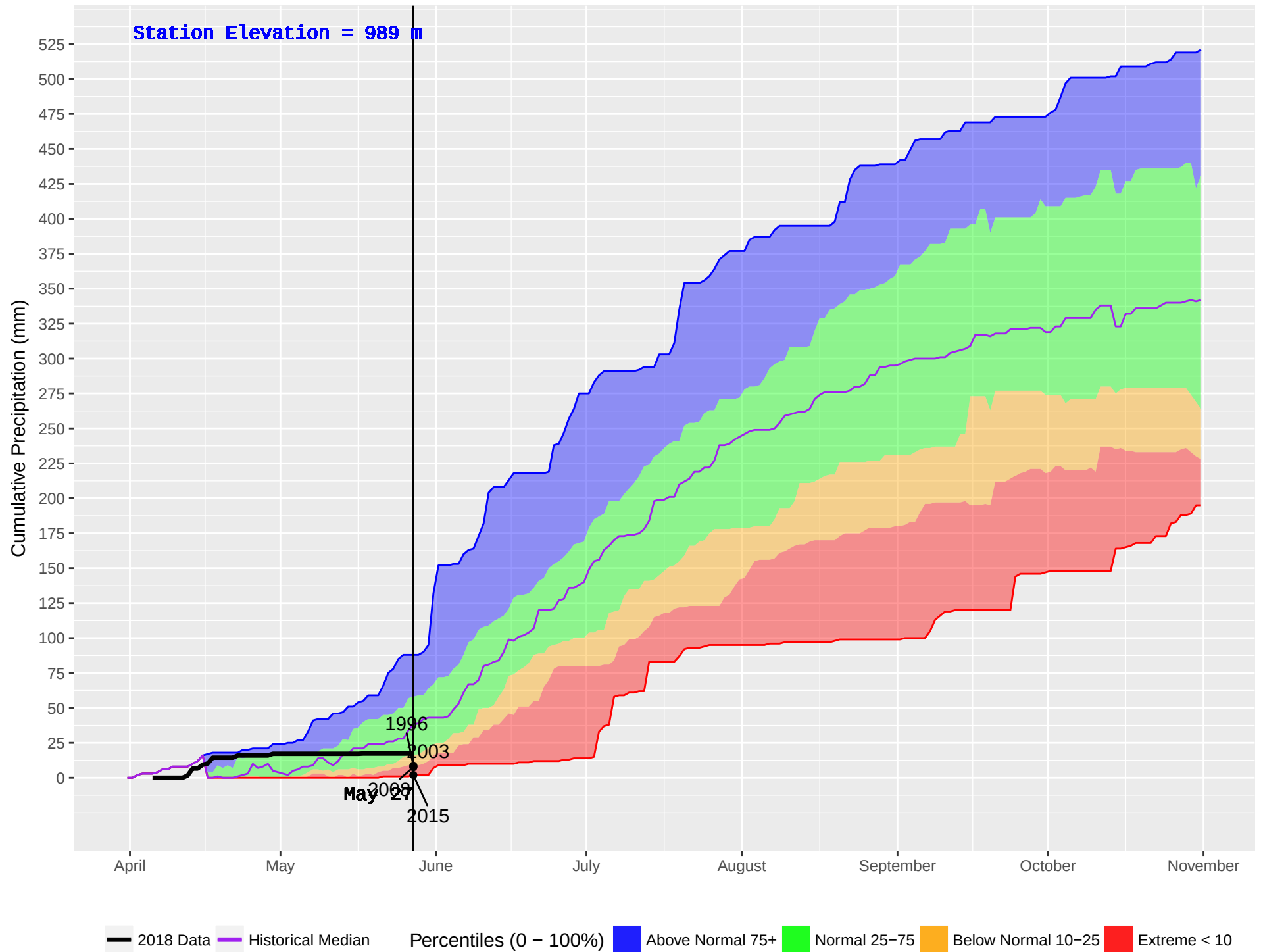
PINK MOUNTAIN (129) : Historical (1983–2016) and Current (2018) Noon Cumulative Precipitation
