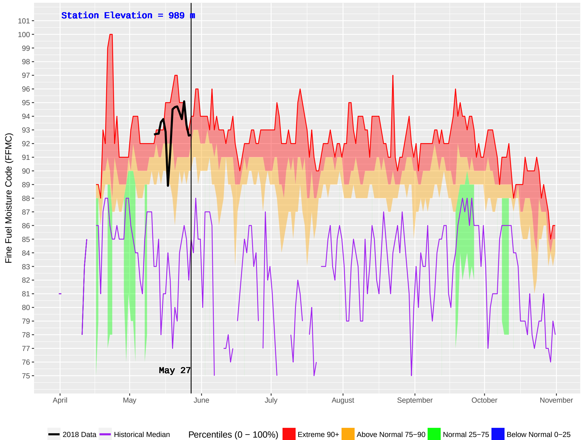
PINK MOUNTAIN (129) : Historical (1983–2016) and Current (2018) Noon Fine Fuel Moisture Code (FFMC)
